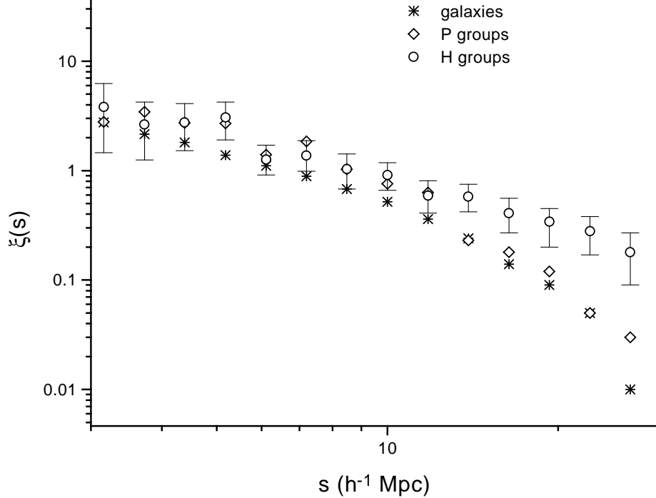
Figure 4: Comparison of the correlation functions for the galaxies, P groups, and H groups; 1\sigma error bars are shown for the H groups only.
